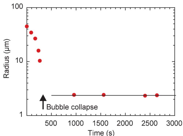
Fig. 3 Typical time evolution of bubble and droplet sizes, observed in the collection chamber of the first experimental configuration described in the text. The bubbles shrink and finally collapse into droplets of constant size. The final stages of the collapse are very fast and could not be resolved in our work using the first experimental configuration. This feature was observed using the second setup described in the text, as illustrated in Fig. 4.
