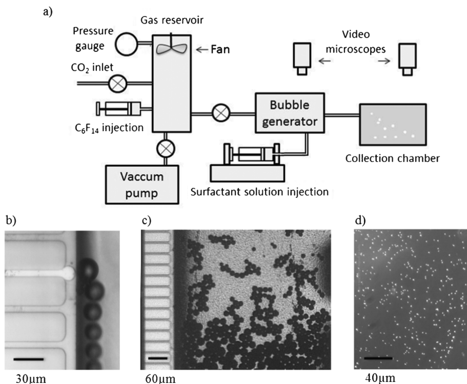
Fig. 2 (a) Schematic view of the experimental setup. (b) Bubble production in a single channel of the micro-fabricated bubble generator. The horizontal channel that looks white is filled with gas and produces bubbles, due to an instability driven by capillary forces. The other horizontal channels are not active in this experiment. (c) Bubble production and onset of shrinkage in the generator. (d) Perfluorocarbon droplets observed in the collection chamber.
