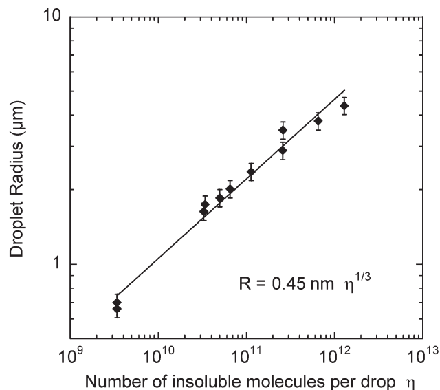
Fig. 5 Final drop radius R obtained after bubble collapse versus the number of water-insoluble molecules \eta initially contained in the bubbles and finally in the drops. The straight line is a power-law fit to the data, as indicated. The drops with a radius below 1 \mu\text{m} were obtained either using the microfabricated bubble generator (initial bubble radius 10 \mu\text{m} ) and the other ones with the flow focusing device (initial bubble radius 45 \mu\text{m} ), as described in the text. The indicated error bars indicated the typical coefficient of variation.
