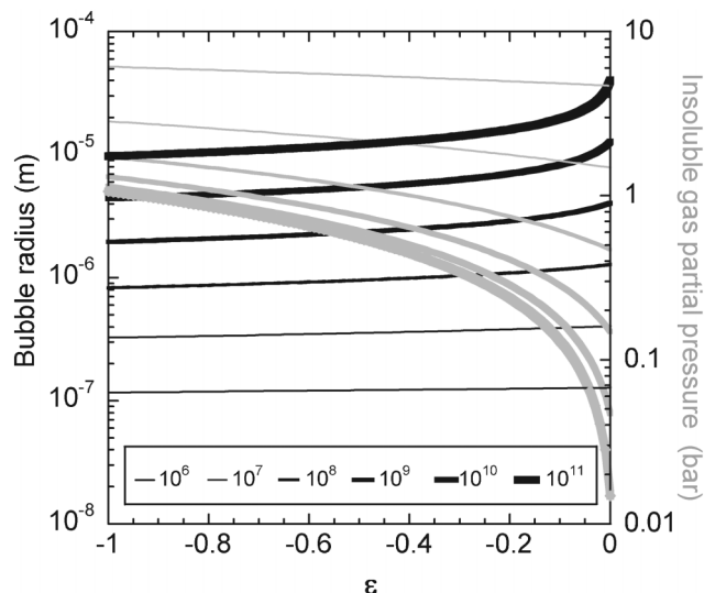
Fig. 1 The equilibrium bubble radius predicted by eqn (1) (black lines) and the partial pressure of the insoluble species (grey lines), considered as an ideal gas, are both plotted versus the degree of saturation \varepsilon of the liquid with the soluble gas, defined in eqn (2). Increasing line thicknesses distinguish the number of insoluble gas molecules per bubble, as specified in the insert. The calculations are performed for a temperature of 298\text{ K} and an interfacial tension of 37.5\text{ mN m}^{-1} .
