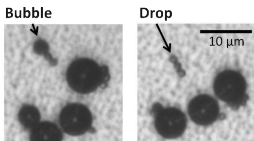
Fig. 4 Two images, taken near the output of the microfabricated foam generator, at a time interval of 5 s illustrate the transformation from bubbles to drops. To avoid convective displacements that carry the bubbles out of the field of view, the gas and liquid injection were stopped just before the observation. Bubbles appear as black disks, whereas drops have a lighter color, as explained in the text.
